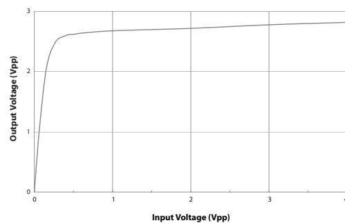
10 MHz distribution amplifier limiter characteristics
